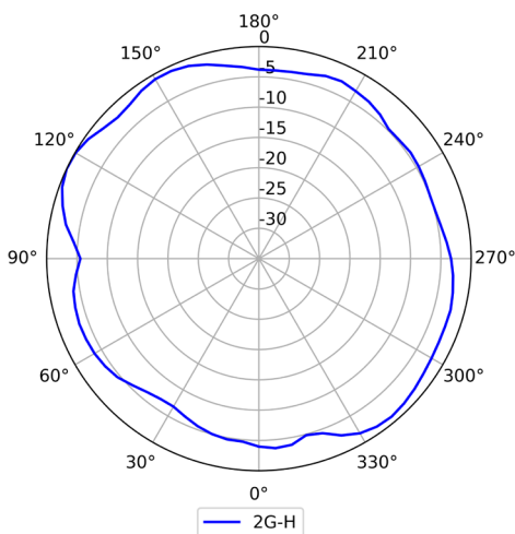
2.4G (Horizontal)
