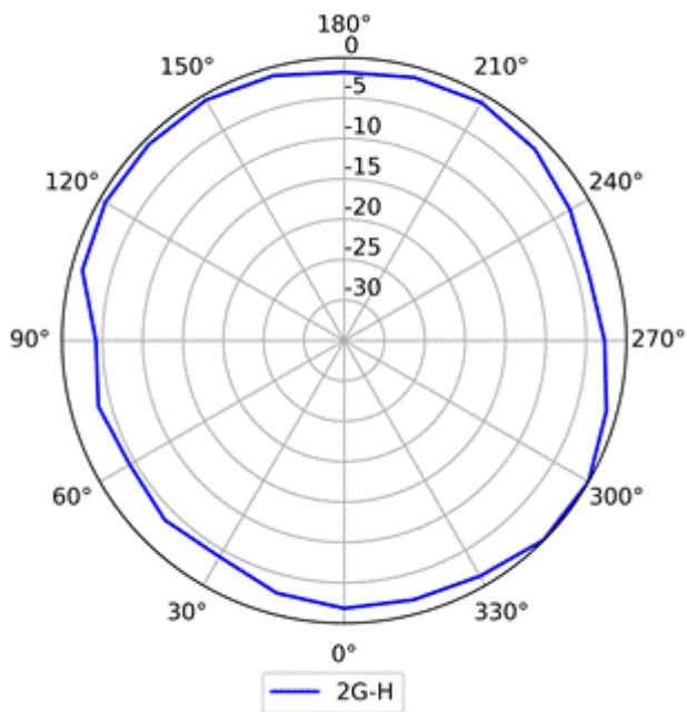
2.4G (Horizontal)
